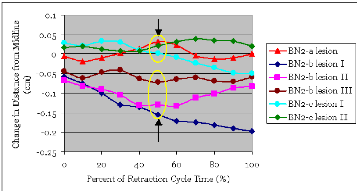
Figure 19. The difference in distance between pre-lesion and post-lesion behavior is plotted along the normalized time scale.
